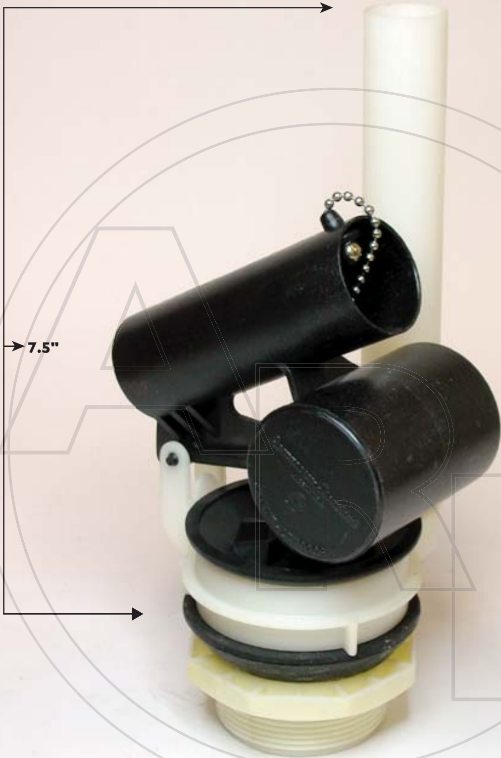
CLOSED CANISTER
