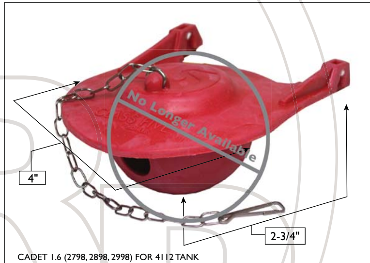
KOH1016546 • FLAPPER NLA USE KOHGP1078441 CHAIN: LINK W/CLIP • CHAIN LENGTH: 7-1/2" O
