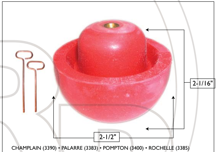
KOHGP88921 • BALL NEW STYLE BALL KIT WITH 2 LIFT RODS
