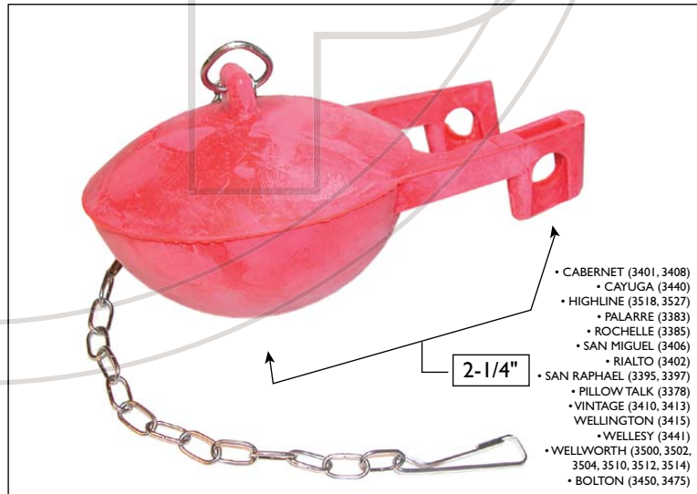
KOHGP49114 • FLAPPER CHAIN: LINK W/CLIP • CHAIN LENGTH: 8"
