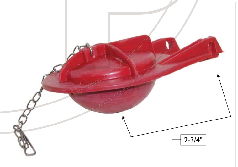
KOHGP1039444 • FLAPPER CHAIN: LINK W/CLIP • CHAIN LENGTH: 5"
